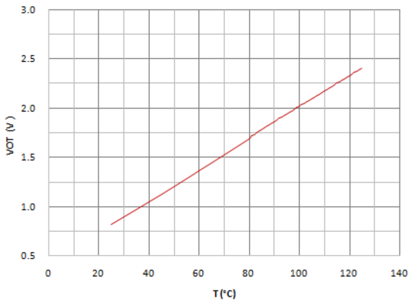
图 5: HVIC 温度检测输出温度—电压曲线 Fig 5: Curves of HVIC Temperature detection-voltage curve
